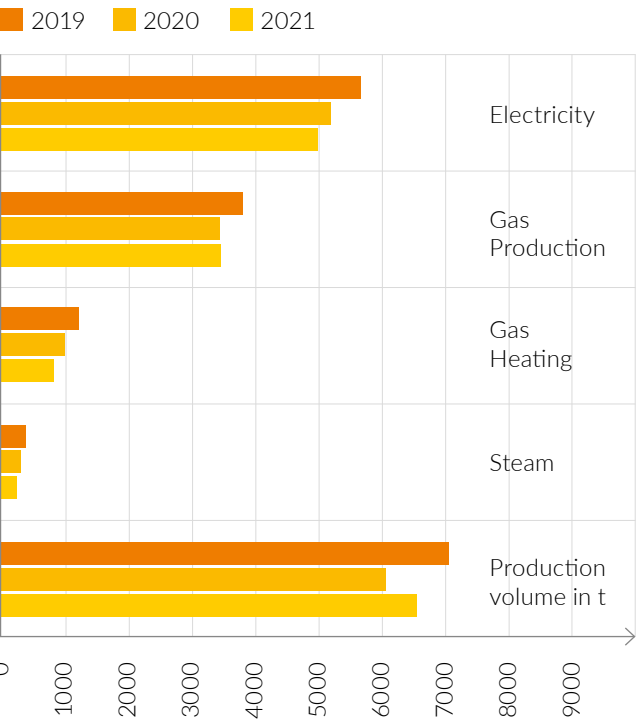
FINAL ENERGY CONSUMPTION IN MWH
